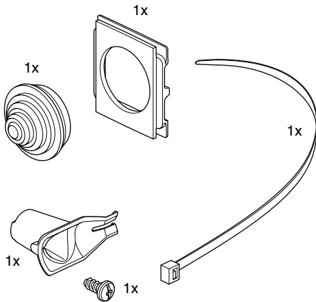
VKG70T
