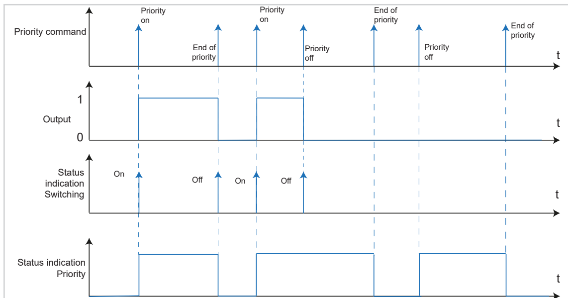
Figure 27: Signal-time diagram for Priority
