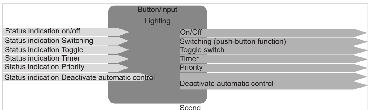
Figure 4: Input/output signals Lighting function
