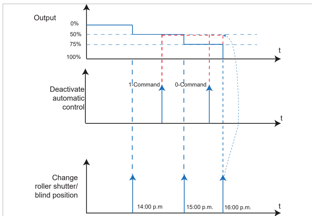
Figure 58: Signal-time diagram for Automatic control deactivation
