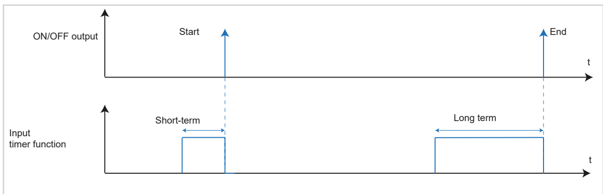
Figure 24: Signal-time diagram for timer
