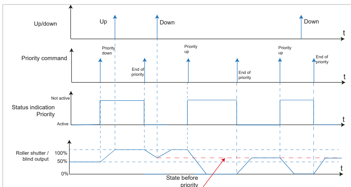
Figure 56: Signal-time diagram for Priority roller shutter/blind
