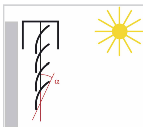
Figure 42: Slat angle at the start of the movement towards the top final position
