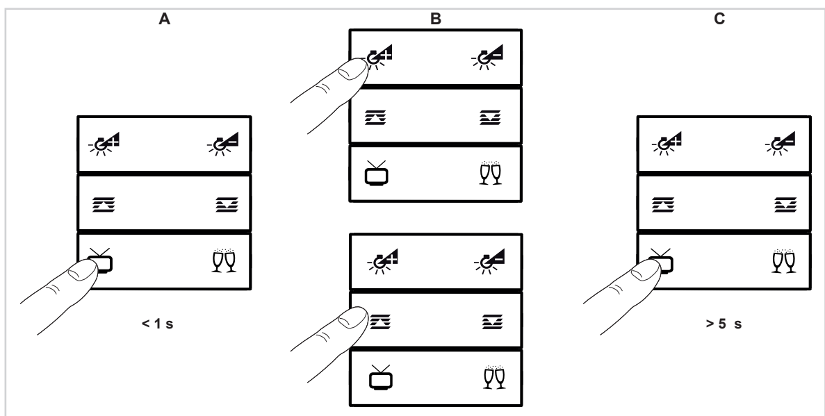
Figure 29: Scene call-up
