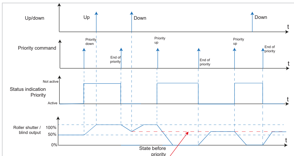
Figure 55: Signal-time diagram for Priority roller shutter/blind
