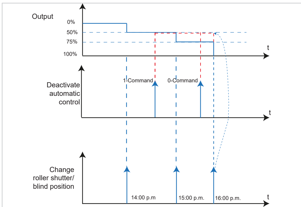
Figure 57: Signal-time diagram for Automatic control deactivation
