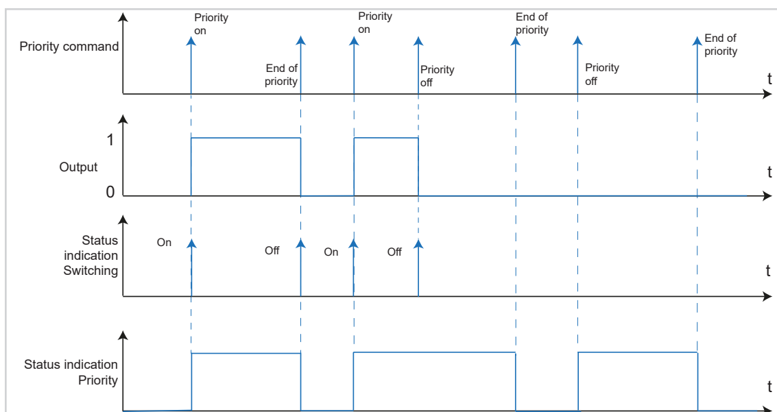
Figure 26: Signal-time diagram for Priority
