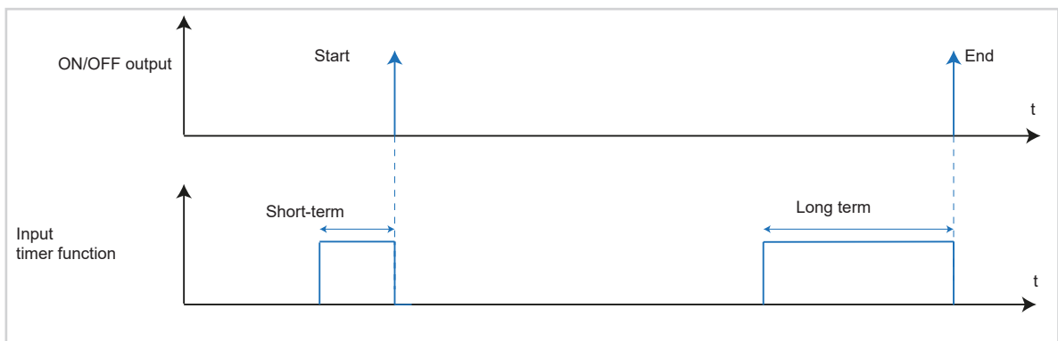
Figure 23: Signal-time diagram for timer
