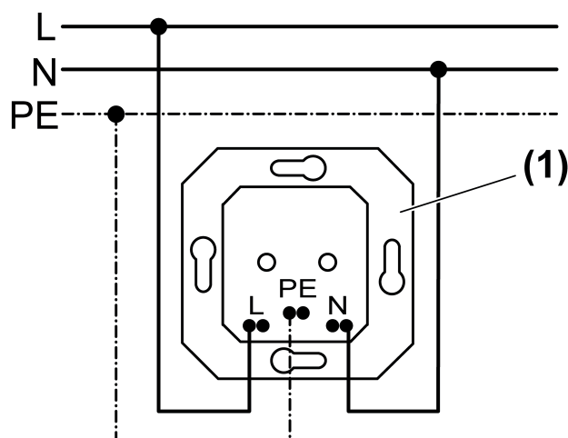
Figure 2: Connection diagram for single socket outlet
