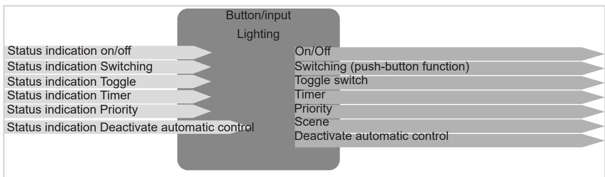
Figure 4: Input/output signals Lighting function
