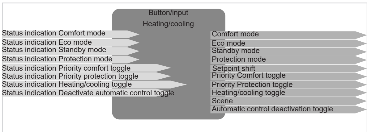
Figure 7: Input/output signals Heating/cooling function
