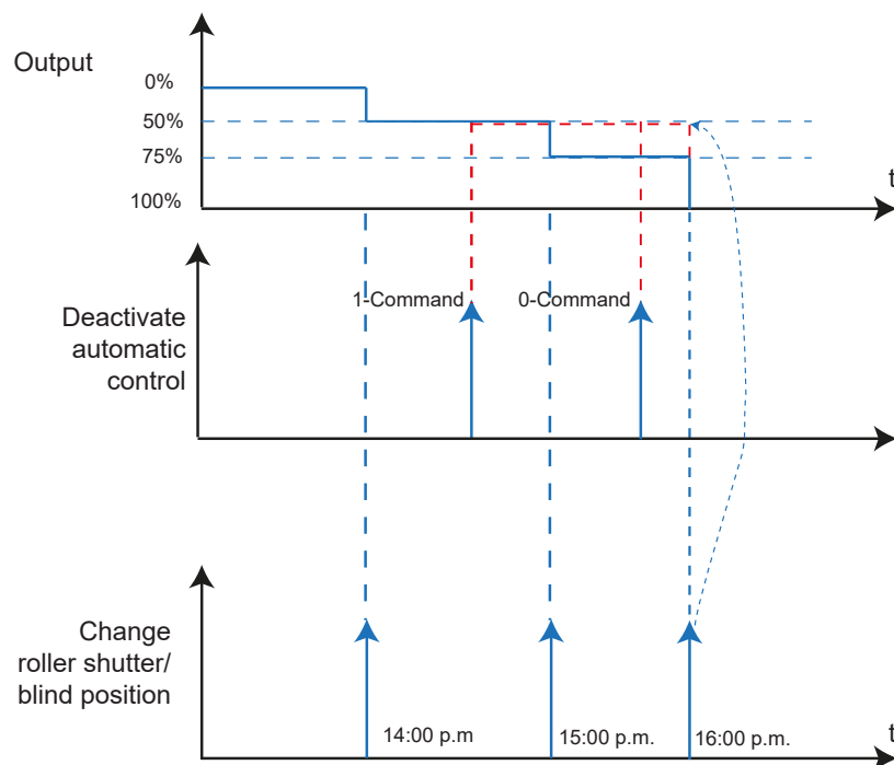
Figure 55: Signal-time diagram for Automatic control deactivation
