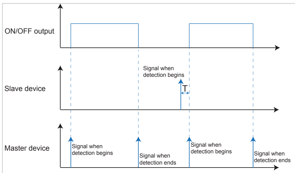
Figure 70: Signal-time diagram for master-slave application
