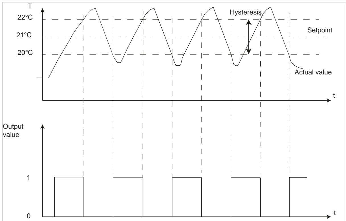
Figure 18: 2-point control
