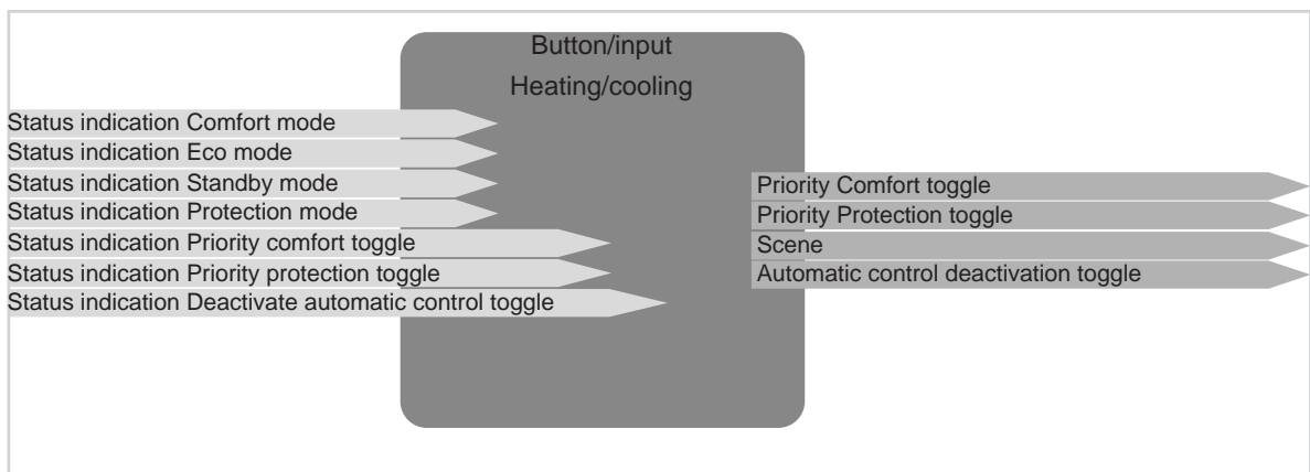
Figure 9: Input/output signals Heating/cooling function
