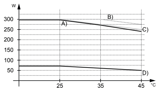
Diagram 1: Maximum output power against ambient temperature
