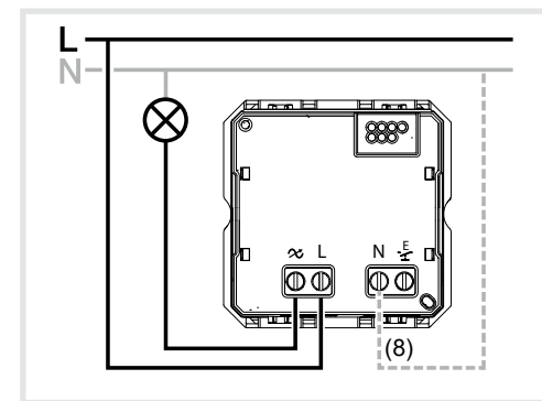
Figure 3: Connecting diagram (basic circuit)
