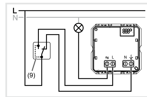
Figure 5: Connecting diagram with change-over switch as extension unit
