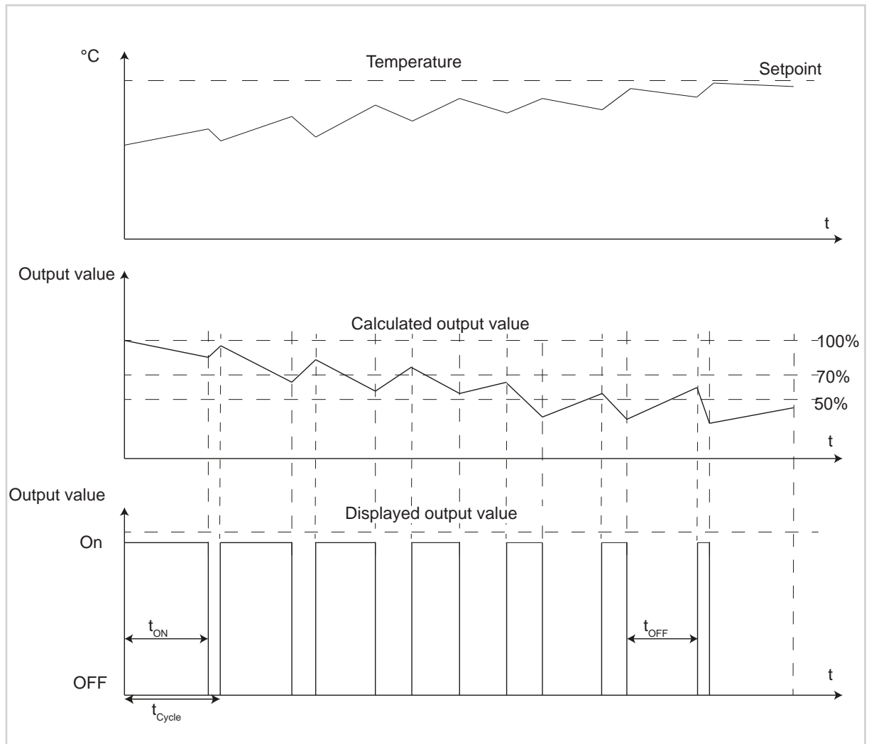
Figure 19: Switching PI-control (PWM)
