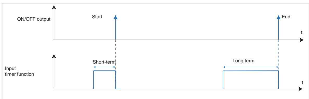
Figure 29: Signal-time diagram for timer
