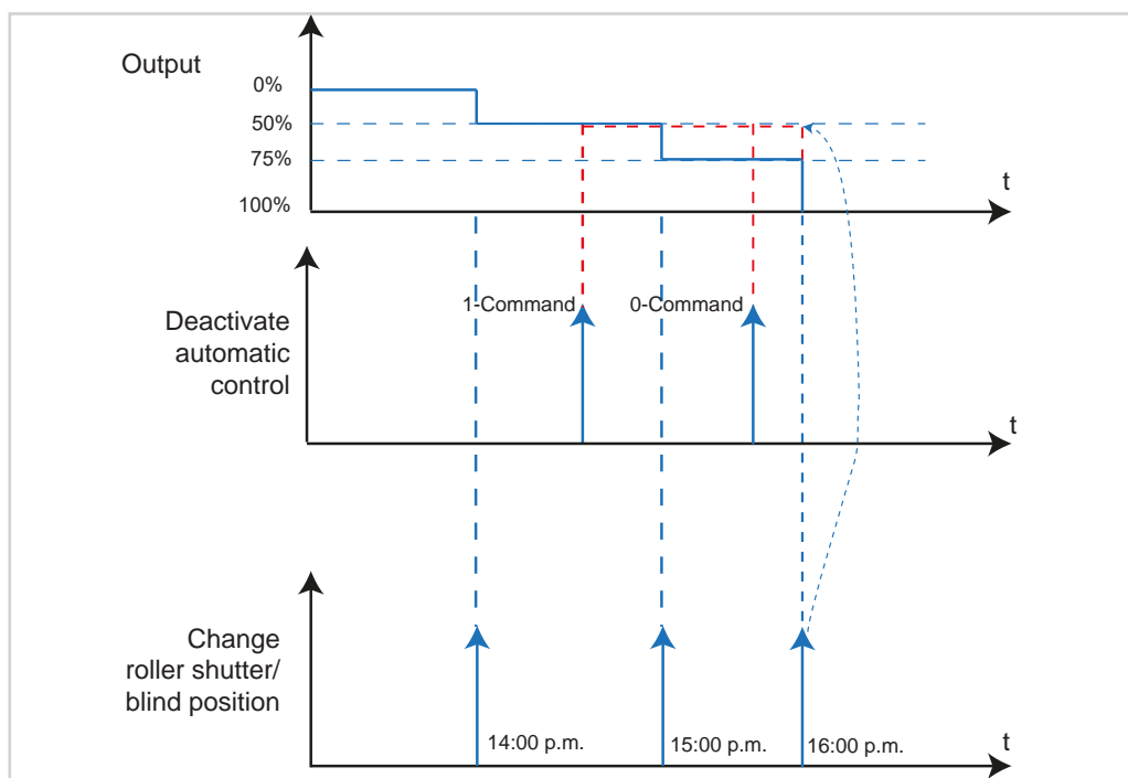
Figure 68: Signal-time diagram for Automatic control deactivation
