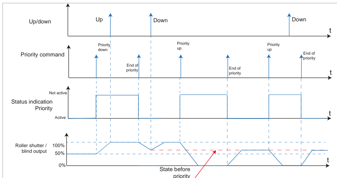
Figure 66: Signal-time diagram for Priority roller shutter/blind
