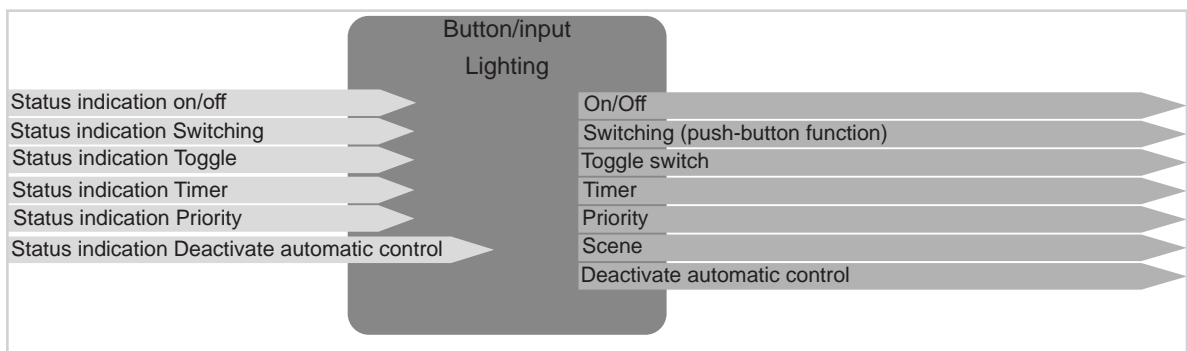
Figure 6: Input/output signals Lighting function
