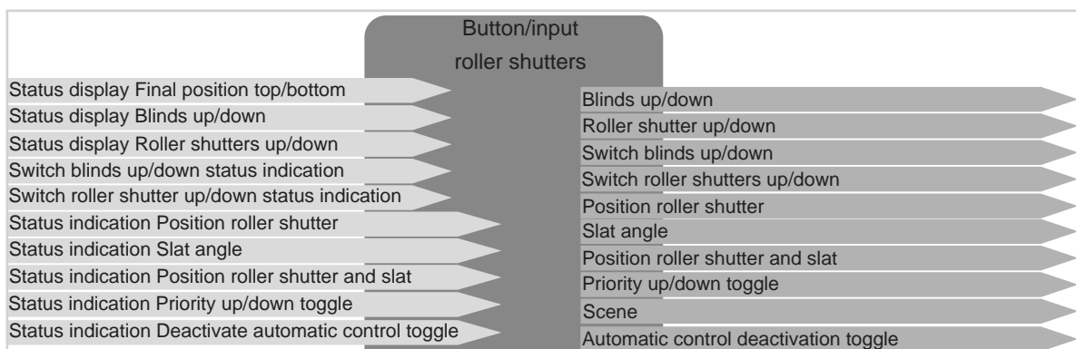
Figure 8: Input/output signals Roller shutter function
