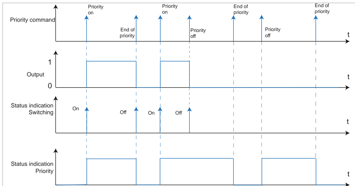
Figure 32: Signal-time diagram for Priority
