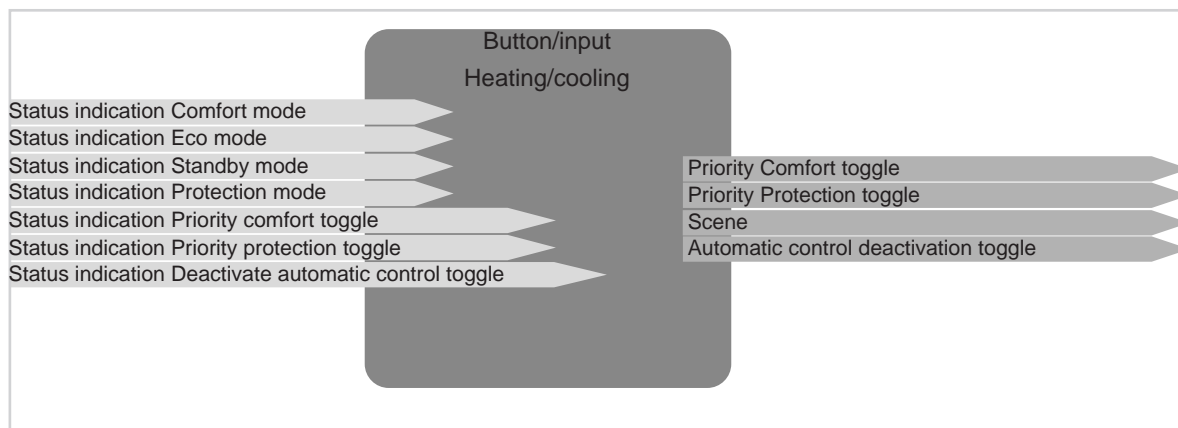
Figure 9: Input/output signals Heating/cooling function
