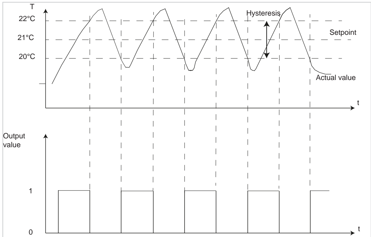
Figure 18: 2-point control
