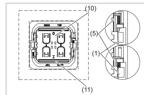
Bild 4: Unlocked and locked radio module
