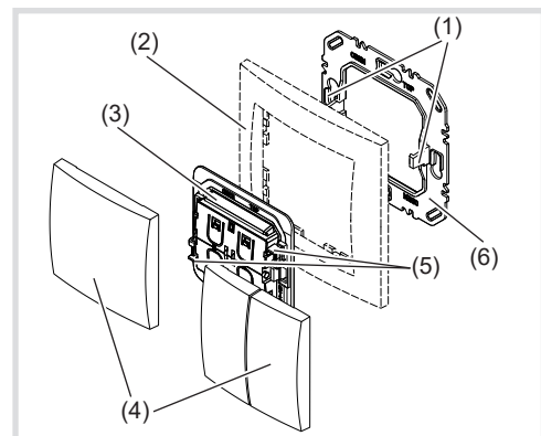
Figure 1: Design and layout of the device wall-transmitter
