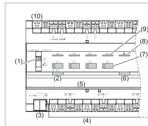
Figure 1 : Device overview
