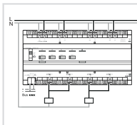
Figure 6 : Output combination (1+2)-(3+4)
