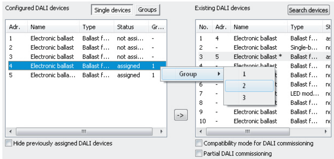
Figure 70: Directly moving assigned devices to another group
