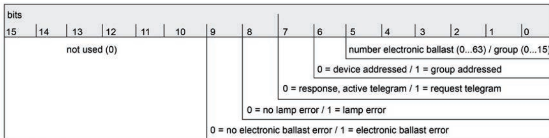
Figure 27: Telegram structure, 2-byte KNX error status
