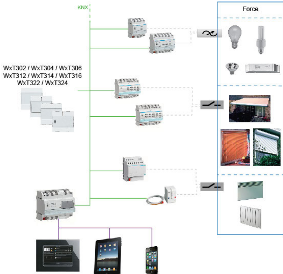
Figure 1: Device overview
