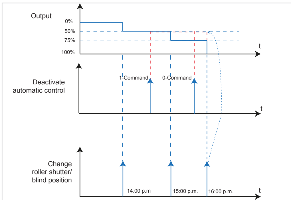
Figure 55: Signal-time diagram for Automatic control deactivation
