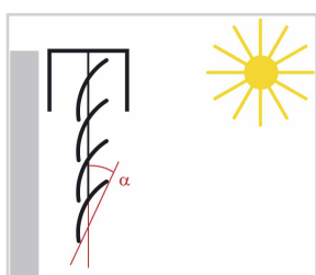
Figure 39: Slat angle at the start of the movement towards the top final position
