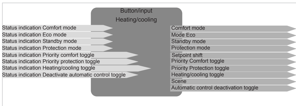
Figure 6: Input/output signals Heating/cooling function
