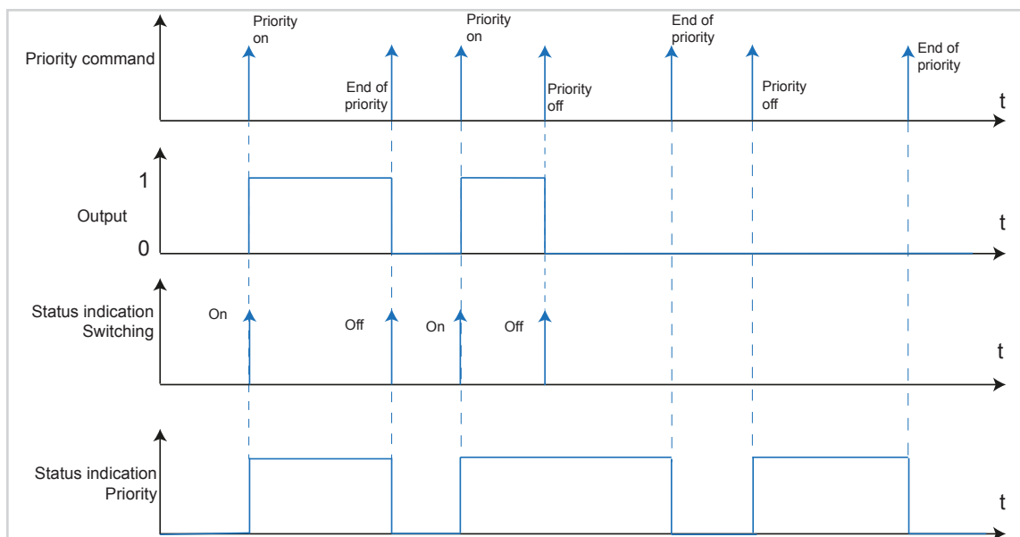
Figure 24: Signal-time diagram for Priority
