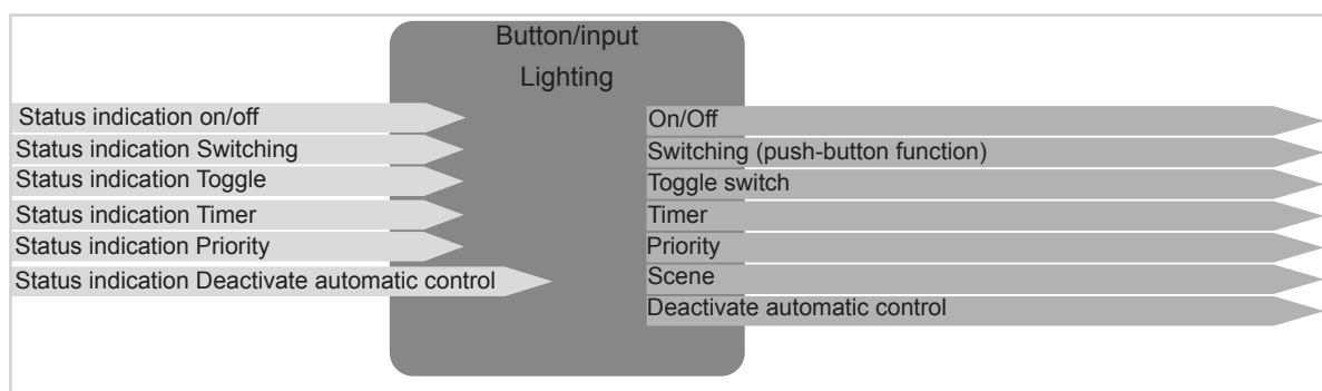
Figure 3: Input/output signals Lighting function
