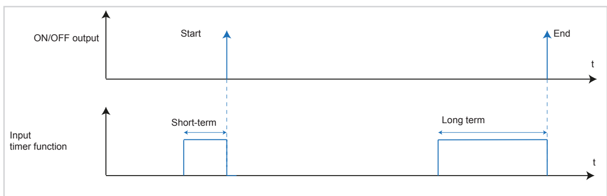
Figure 21: Signal-time diagram for timer
