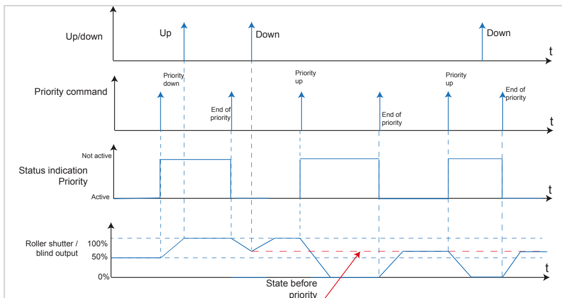
Figure 53: Signal-time diagram for Priority roller shutter/blind
