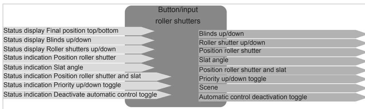
Figure 5: Input/output signals Roller shutter function
