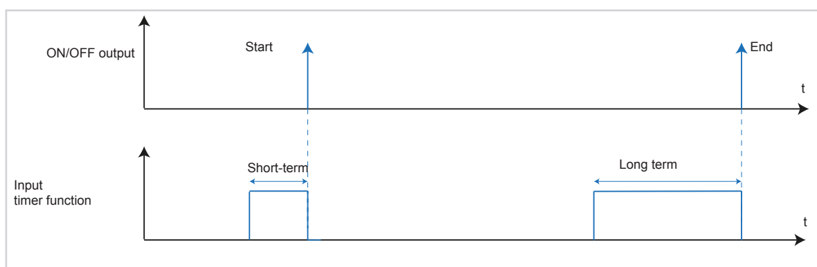
Figure 19: Signal-time diagram for timer
