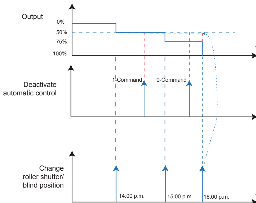
Figure 53: Signal-time diagram for Automatic control deactivation
