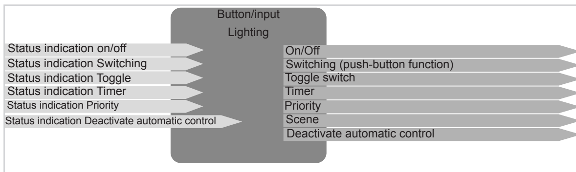
Figure 4: Input/output signals Lighting function
