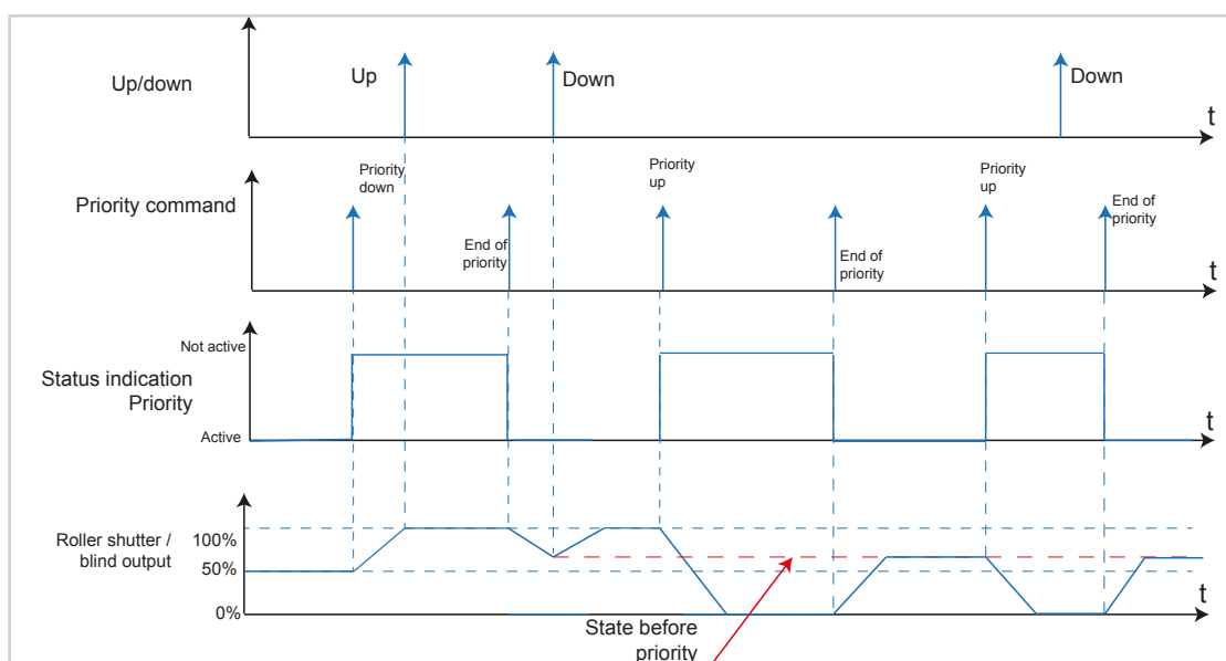
Figure 51: Signal-time diagram for Priority roller shutter/blind
