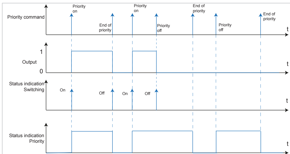
Figure 22: Signal-time diagram for Priority
