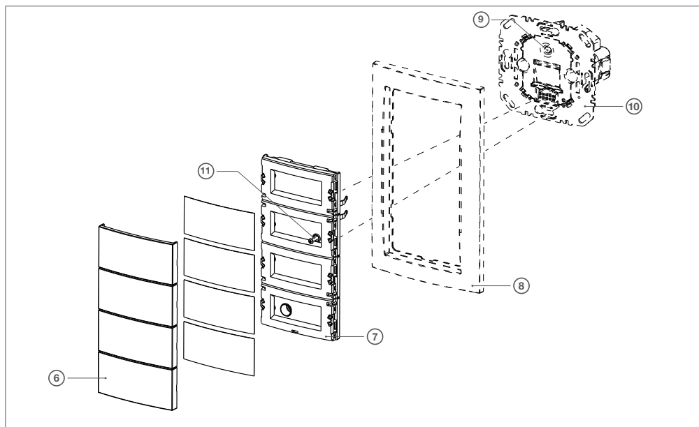
Figure 3: Assembly of the device
