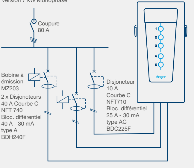
Coffret de protection. Version 7 kW Monophasé
