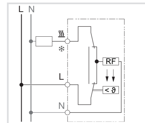
Figure 4: Electrical connection
