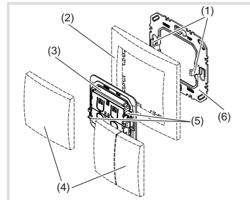
Figure 1: Design and layout of the device wall-transmitter
