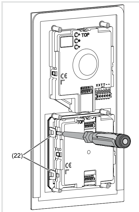
Figure 20: Unlatching module
