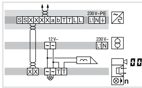
Figure 8: Door release connection on the door station
