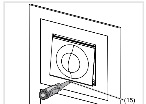
Figure 10: Dismantling video module centre plate
