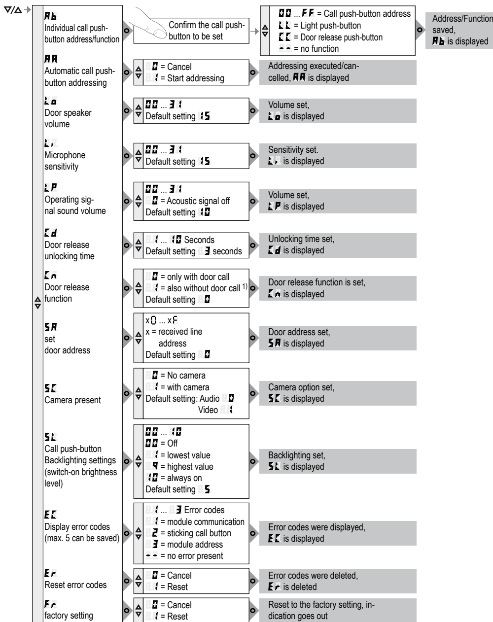
Figure 9: Overview of system settings
