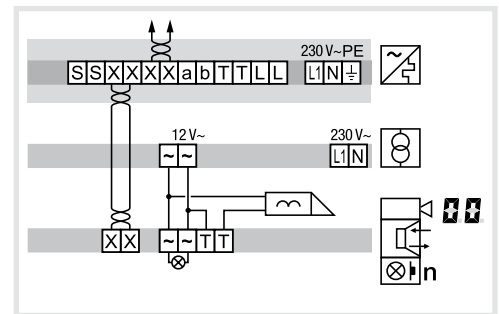
Figure 6: Door release connection on the door station
