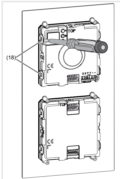
Figure 17: Unlatching module
