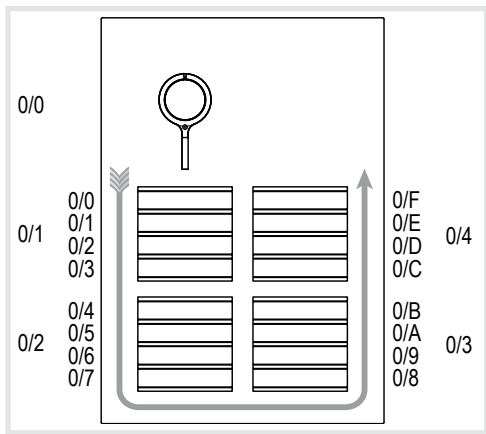
Figure 8: Module address and automatic call push-button addressing
