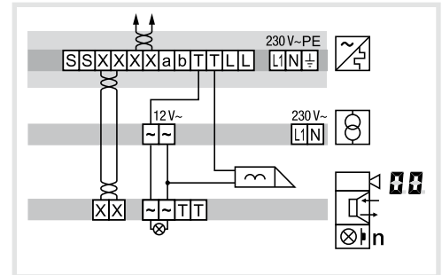
Figure 7: Connection of door station video with manipulation-protected door release
