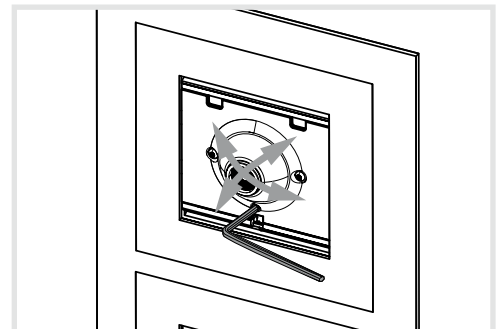
Figure 11: Camera alignment video module
