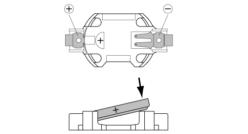
Figure 5: Insert battery
