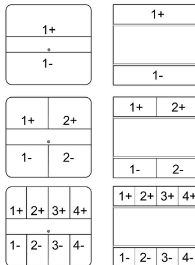
picture 3: Channel assignment 1-gang, 2-gang, 4-gang
