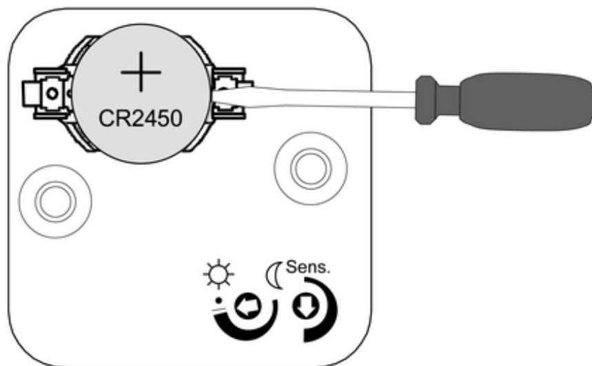
picture 7: Remove battery
