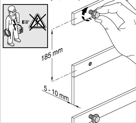
Montageart 1; Spannungsfrei Kind of assembly 1; Zero potential
