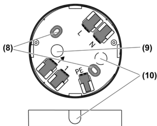
picture 5: Connection box
