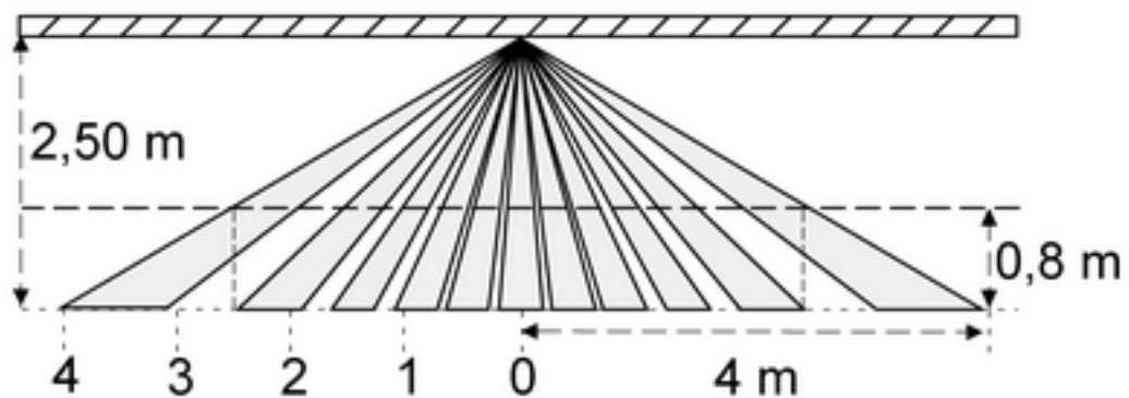
picture 3: Detection field
