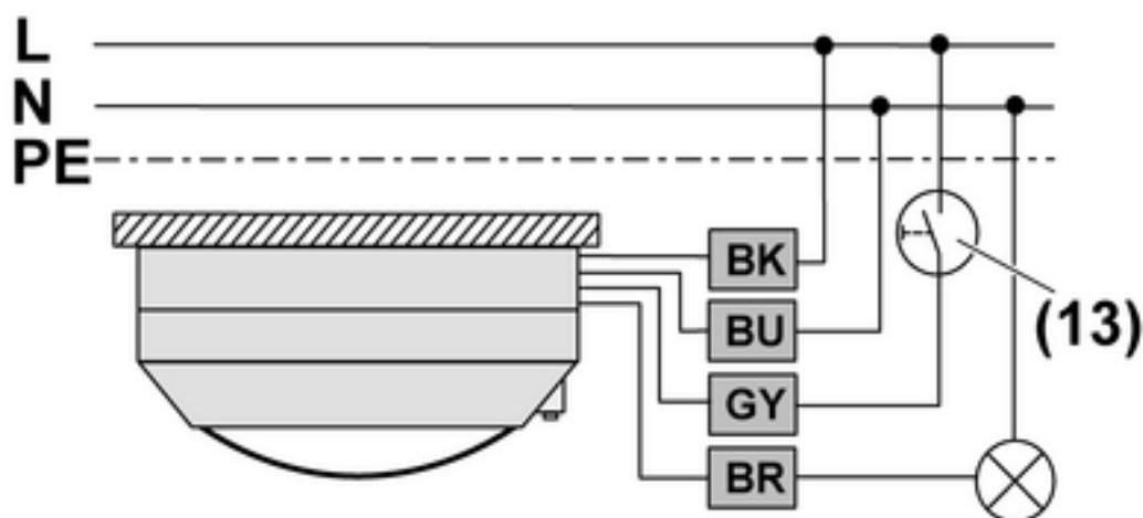
picture 6: Connection diagram
