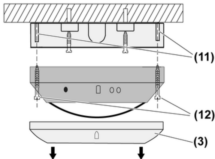
picture 4: mounting
