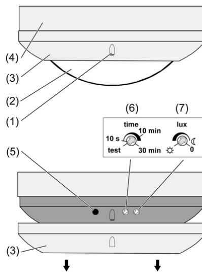
picture 1: Device components
