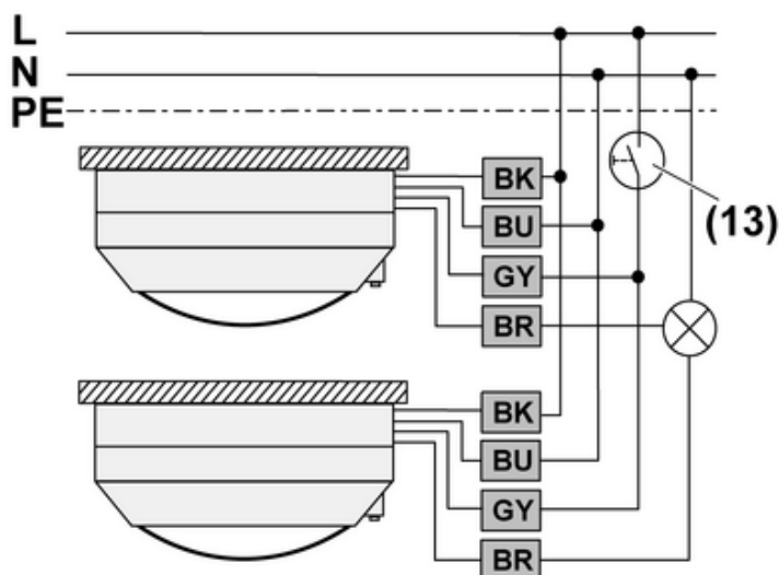
picture 7: Connection diagram for connection in parallel
