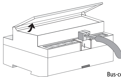
Bus-connection
