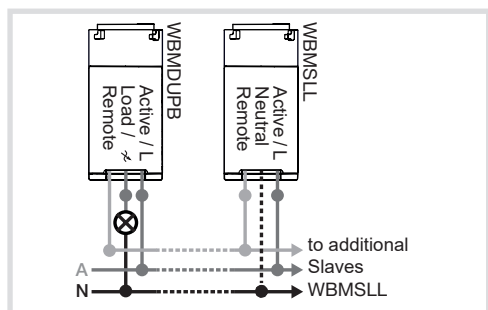
Fig. 5: 2 way connection
