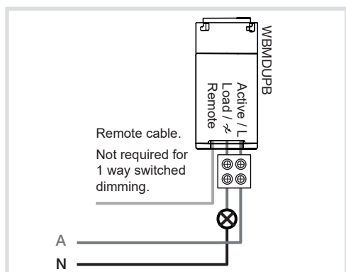
Fig. 4: 1 way connection
