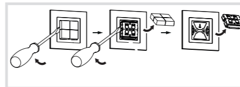
Figure 7: Dismantling
