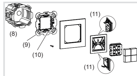
Figure 5: Installation on a wall box
