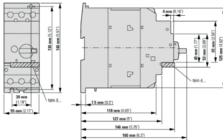
Image 40: Motor protection switch size 2
