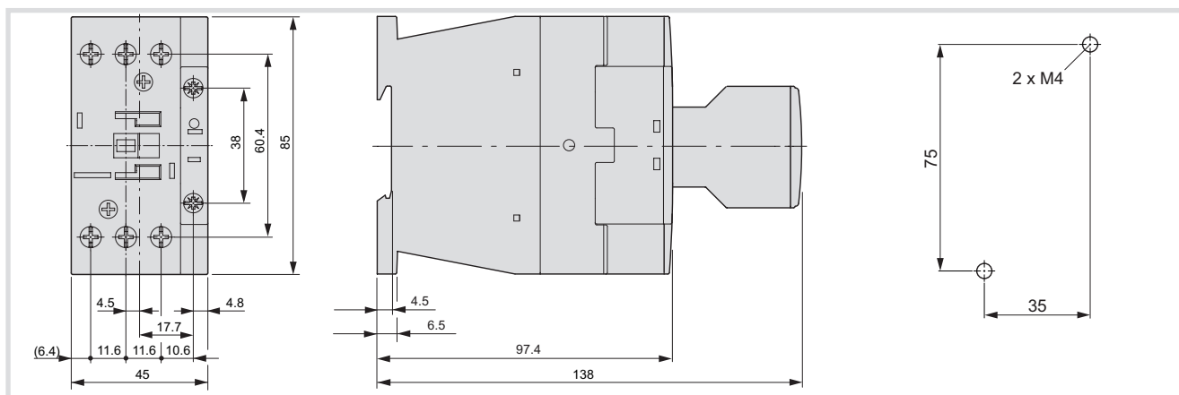
Image 34: Lamp contactor dimensions
