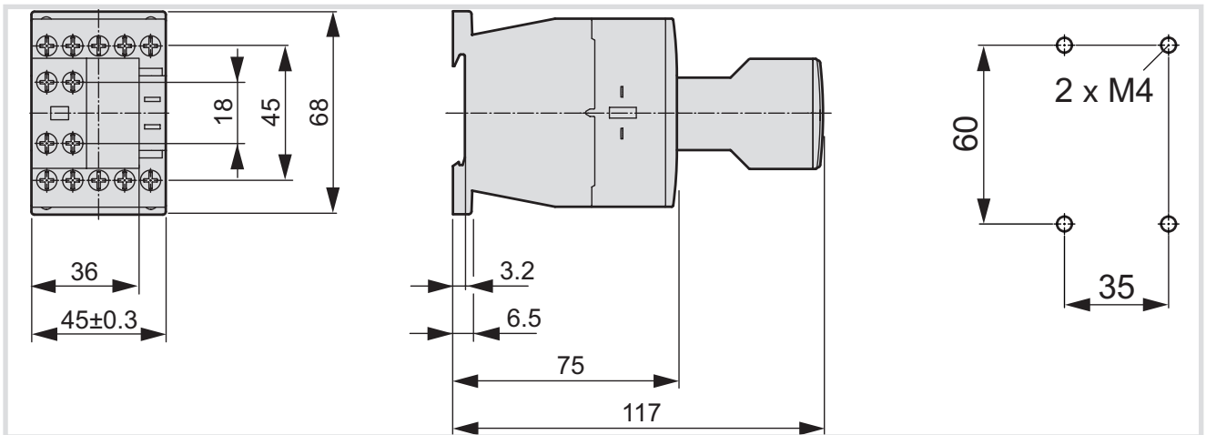
Image 30: 4pole power contactors (EVN022)
