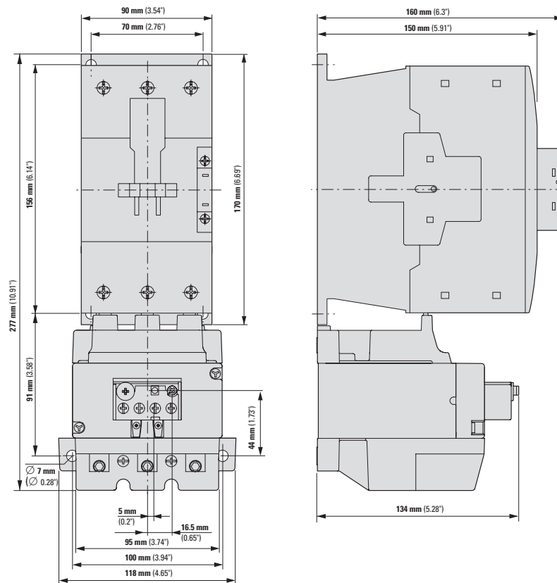
Image 38: EVBxxxD
