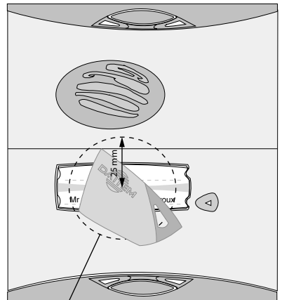
The tag is detected in this zone at a maximum distance of 20 mm.
