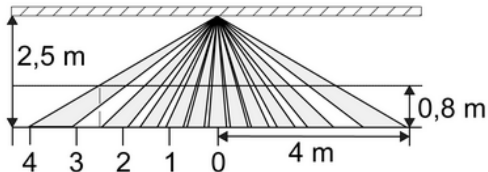
Figure 5: Detection area
