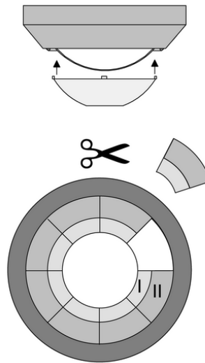
Figure 12: Push-on cover
