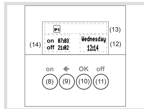
Figure 2: Display and operating elements
