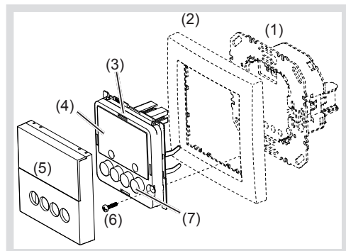
Figure 1: Design of the device
