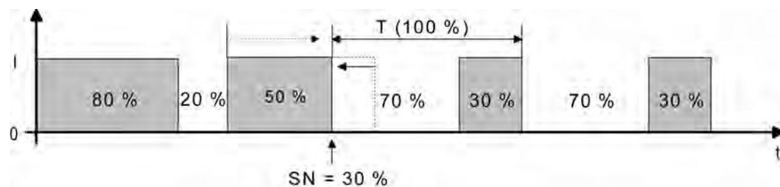
picture 19: Command value change, e.g. from 80 % to 30 % during the opening phase of the valve (opening phase too long)
