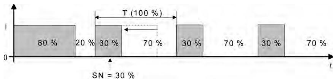
picture 17: Command value change, e.g. from 80 % to 30 % during the opening phase of the valve
