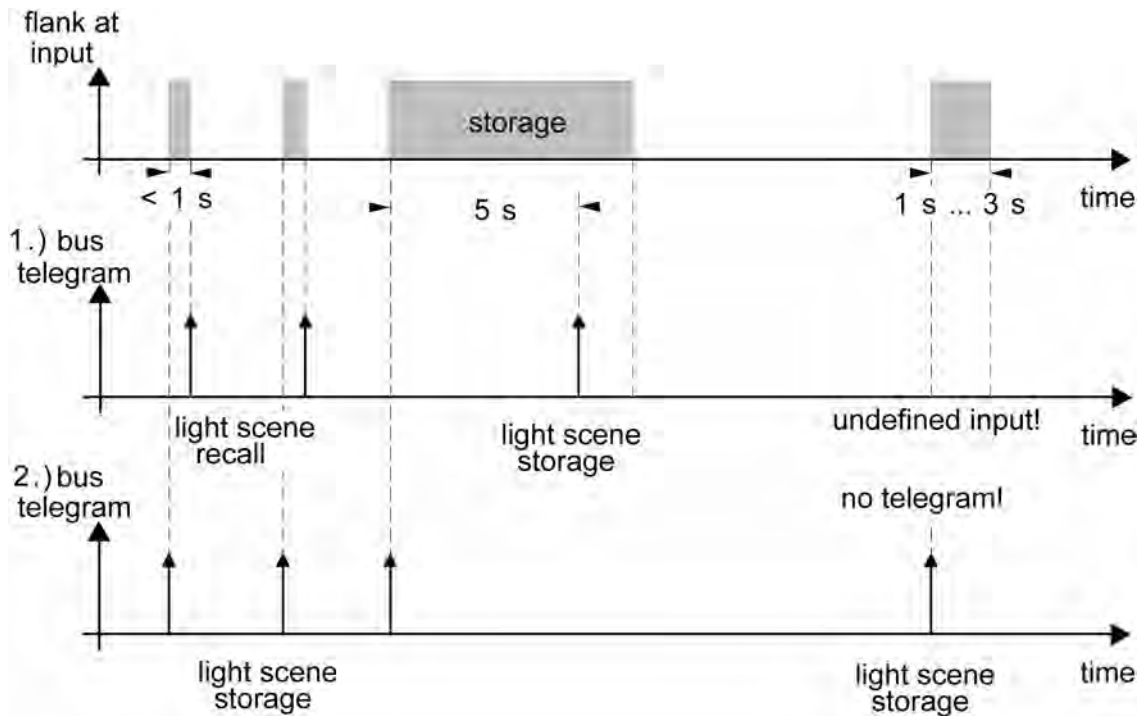
picture 9: Example of scene storage
