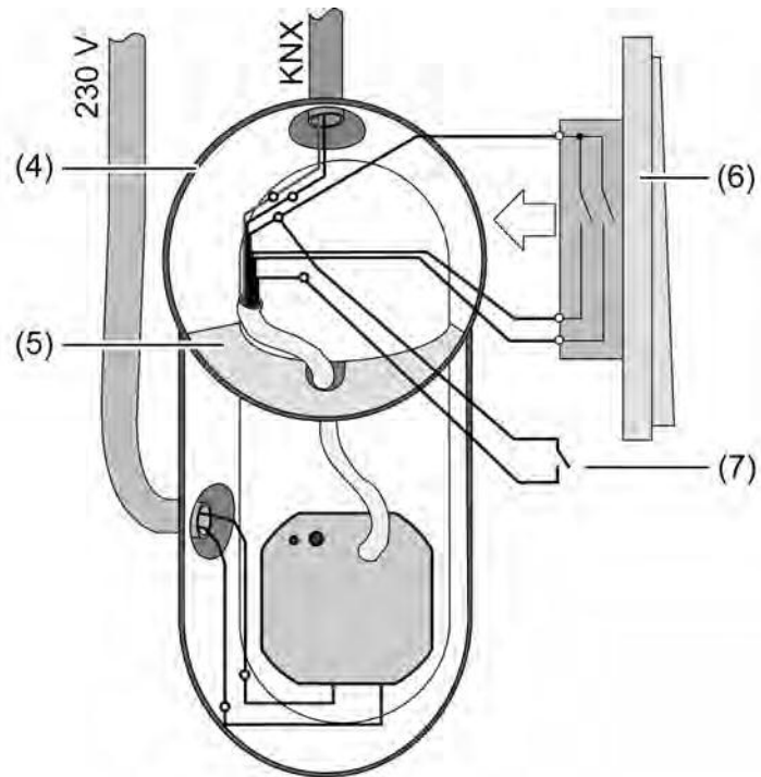
picture 3: Installing the device in an electronics box (example)
