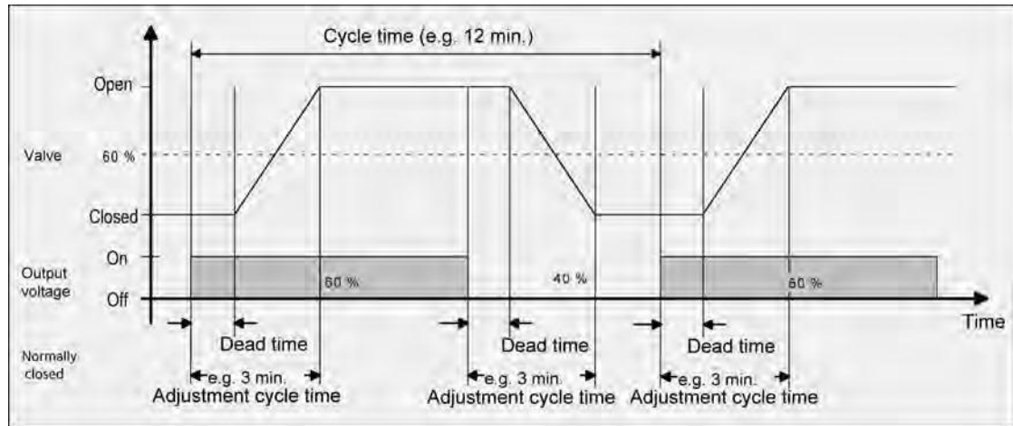
picture 23: Ideal course of the valve stroke for a command value of approx. 60 % of a deenergised, closed valve
