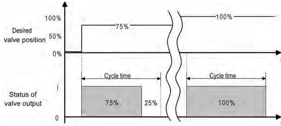
picture 11: Conversion of a constant valve setpoint position to an output signal with deenergised, closed valve drives (example)
