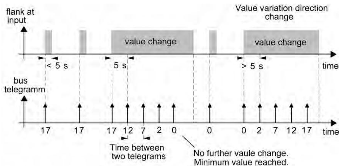
picture 8: Example to change the value for dimming value encoder
