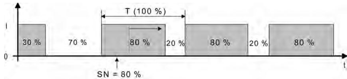
picture 20: Command value change, e.g. from 30 % to 80 % during the opening phase of the valve
