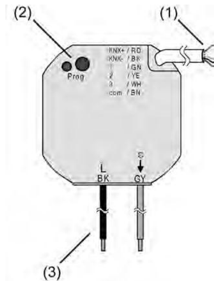
Picture 1: Device components
