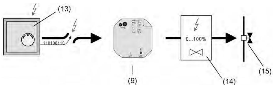
picture 25: Principle of cyclical command value monitoring in the event of a fault (e.g. open circuit)
