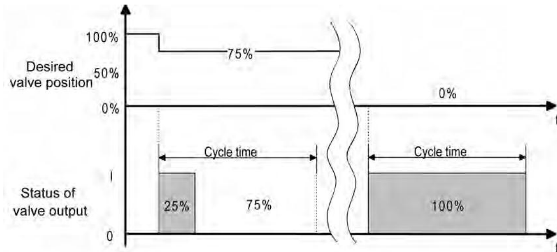
picture 13: Conversion of a constant valve setpoint position to an output signal with deenergised, opened valve drives (example)
