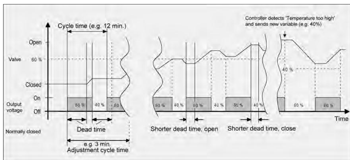
picture 24: Ideal course of the valve stroke for a command value of approx. 60 % at first of a deenergised, closed valve
