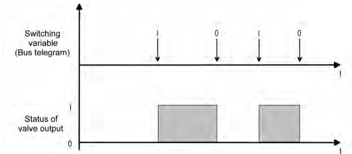
picture 10: Conversion of a switching command value to an output signal with deenergised, closed valve drives (example)
