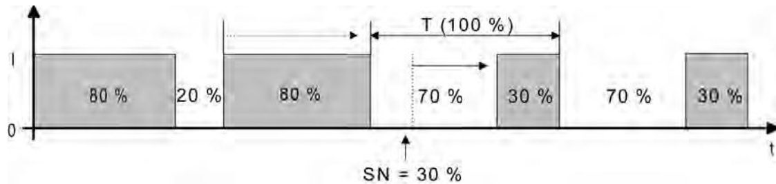
picture 18: Command value change, e.g. from 80 % to 30 % during the closing phase of the valve
