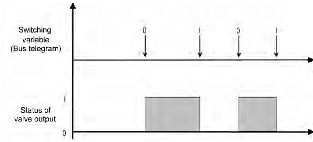
picture 12: Conversion of a switching command value to an output signal with deenergised, opened valve drives (example)
