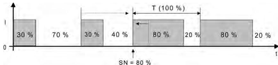
picture 22: Command value change, e.g. from 30 % to 80 % during the closing phase of the valve (closing phase too long)
