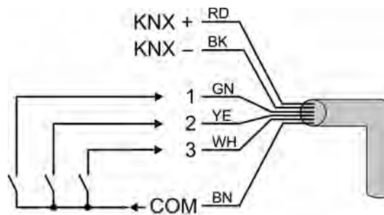
picture 5: Connection of the extension inputs
