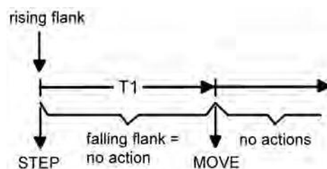
picture 7: Operation concept "long – short"
