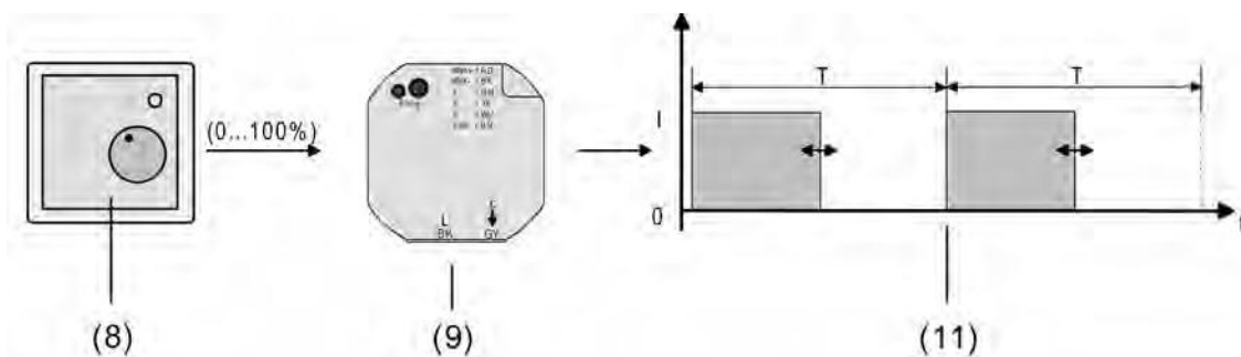
picture 15: Command value principle for constant command value
