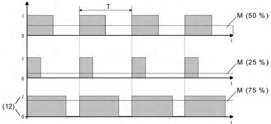
picture 16: Pulse width modulation of a valve output signal
