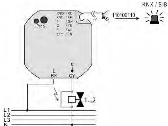
picture 26: Short-circuit and overload detection in case of fault in valve output or valve drive
