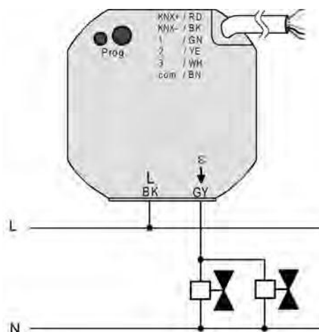
picture 4: Connection of the mains voltage and the load
