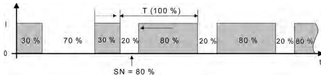
picture 21: Command value change, e.g. from 30 % to 80 % during the closing phase of the valve
