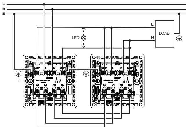
1gang 2way DP switch w/LED
