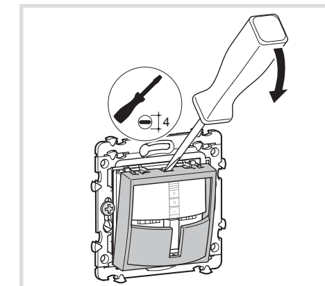
Figure 8: Dismantling of cover
