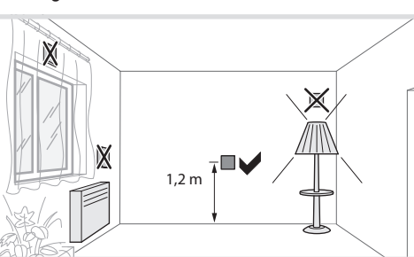
Figure 7: Installation location of the motion detectors
