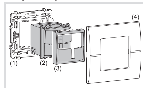
Figure 1: Design and layout of the device
