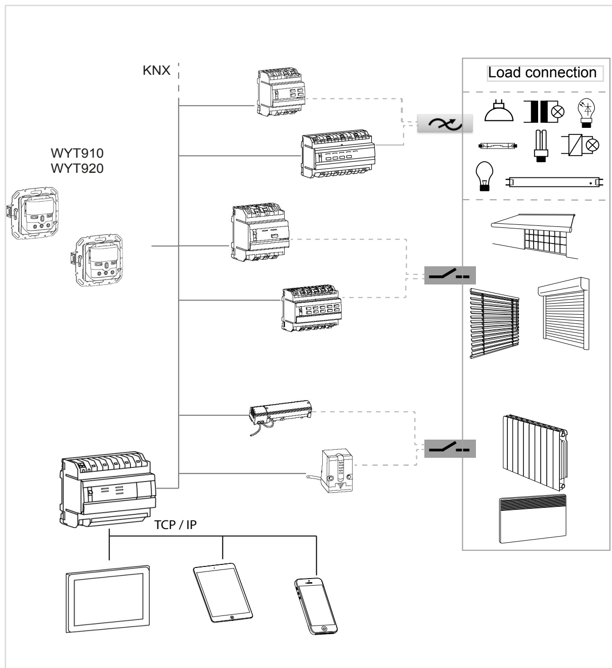
Figure 1: Device overview
