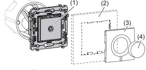
Figure 2: WK061 touch dimmer
