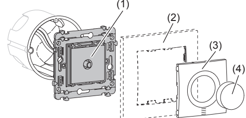
Figure 1: WK060 rotary dimmer
