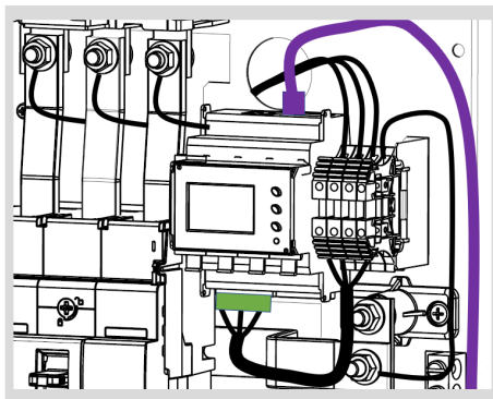
Fit meter sub-assembly to support bracket and connect the meter L1 L2 L3 ring terminals to the M8 studs and torque to 13Nm, connect the Neutral cable to the neutral assembly and re-torque to 13Nm.
