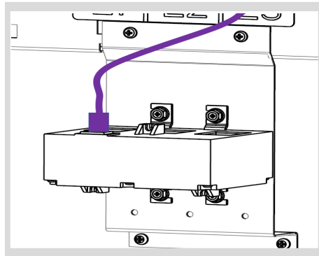
Fit lower CT pack to pan assembly using 2 x M4 m/c screws and 2x self tapping screws. Plug RJ45 lead into CT & meter.
