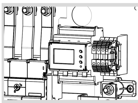
Fit the meter and fuses back in place as shown above.
