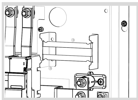
Fit 2 x meter bracket M4 fixings into the chassis, allowing clearance for the bracket slots
