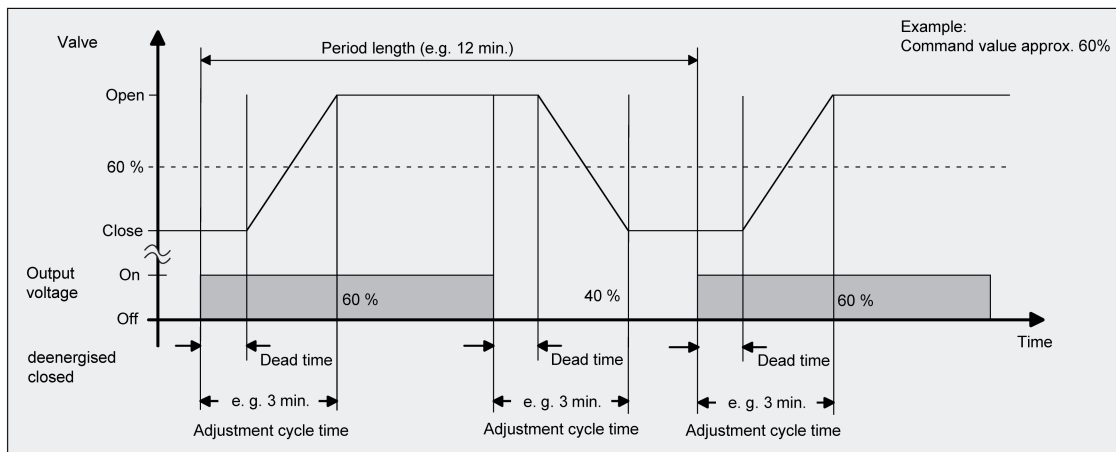
Figure 17: Ideal course of the valve stroke for a cycle time > 2 \times Adjustment cycle time
