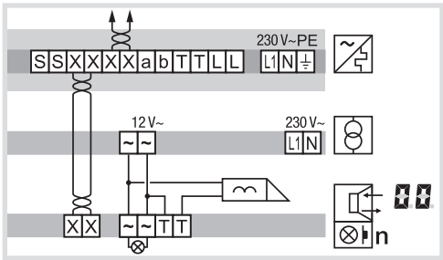
Figure 7: Door release station on the device
