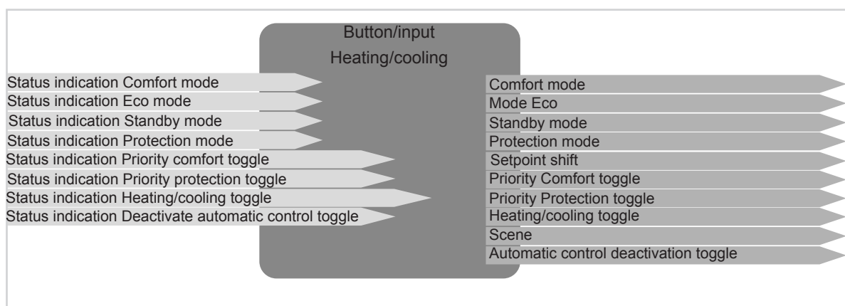
Figure 6: Input/output signals Heating/cooling function
