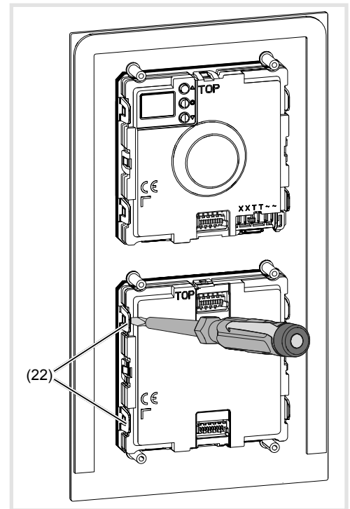
Figure 17: Unlatching module
