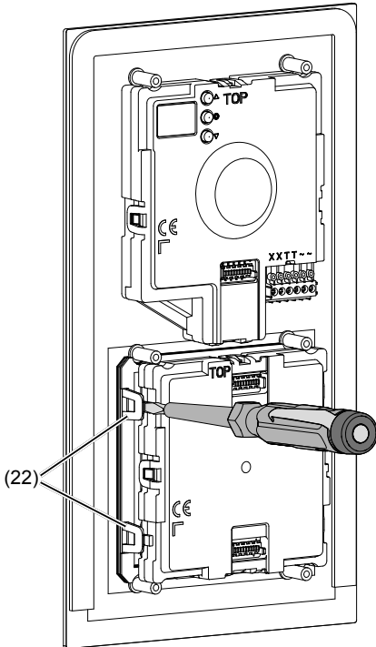
Figure 20: Unlatching module
