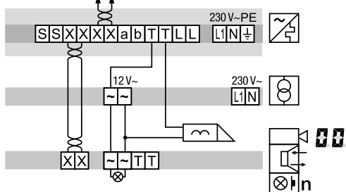
Figure 9: Connection of door station video with manipulation-protected door release
