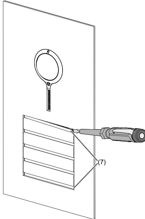
Figure 16: Removal of cover strips
