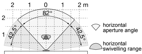
Figure 15: Horizontal camera orientation
