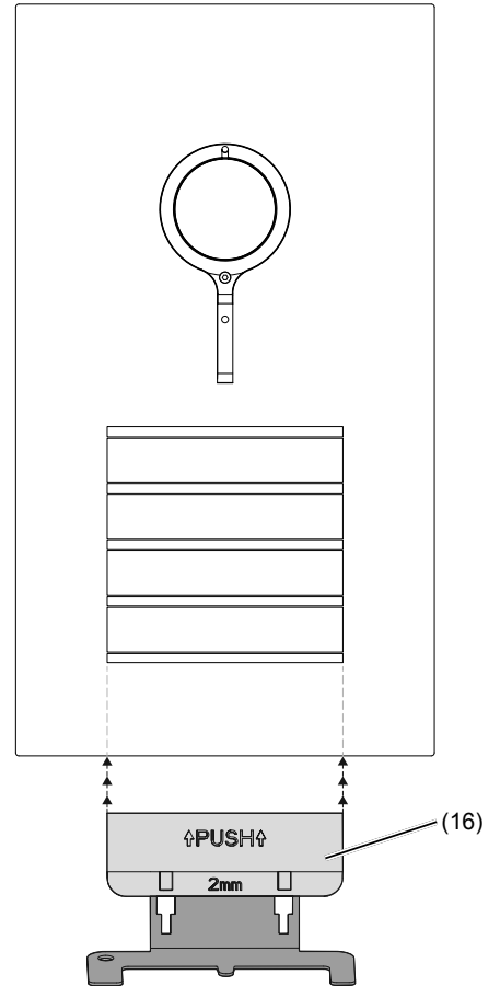
Figure 18: Opening of the door station
