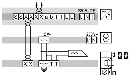
Figure 8: Door release connection on the door station
