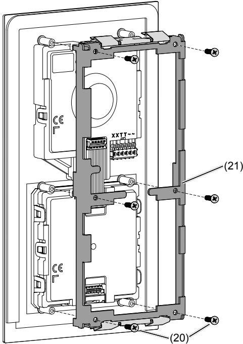
Figure 19: Dismantling module mounting
