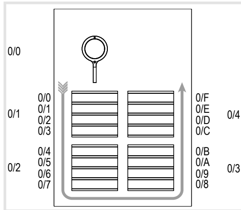
Figure 11: Module address and automatic call push-button addressing
