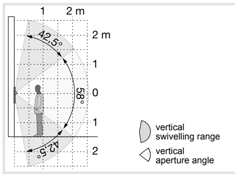
Figure 14: Vertical camera orientation
