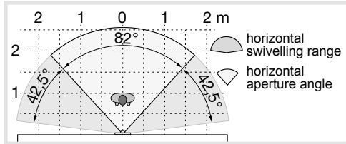
Figure 15: Horizontal camera orientation
