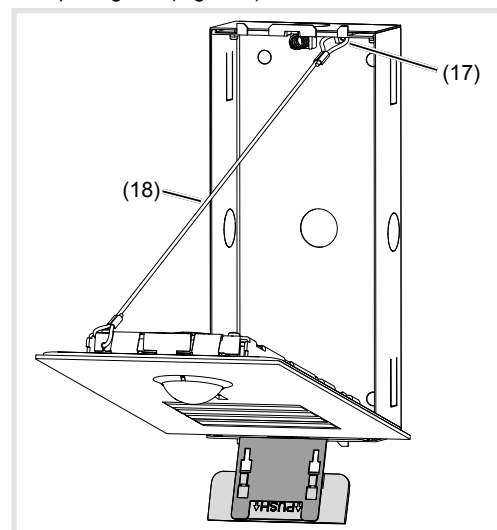
Figure 6: installation position of door station
