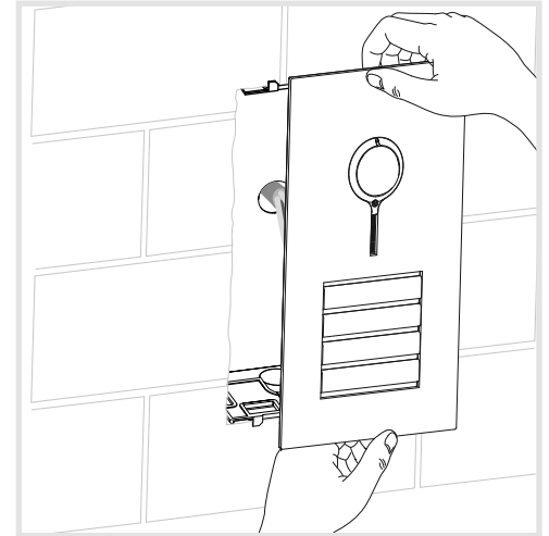
Figure 12: Insert door station
