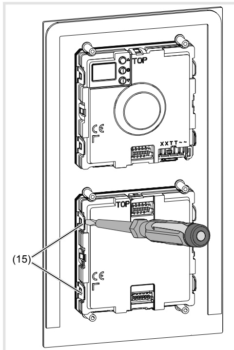
Figure 13: Unlatching module
