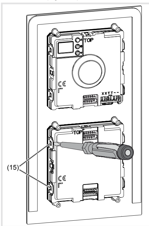
Figure 13: Unlatching module
