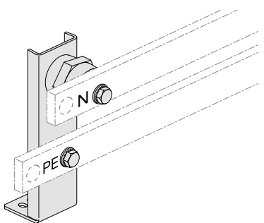
univers N UST42PEN
