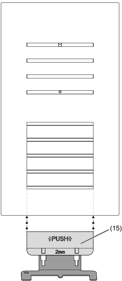
Figure 15: Disassembling the door station
