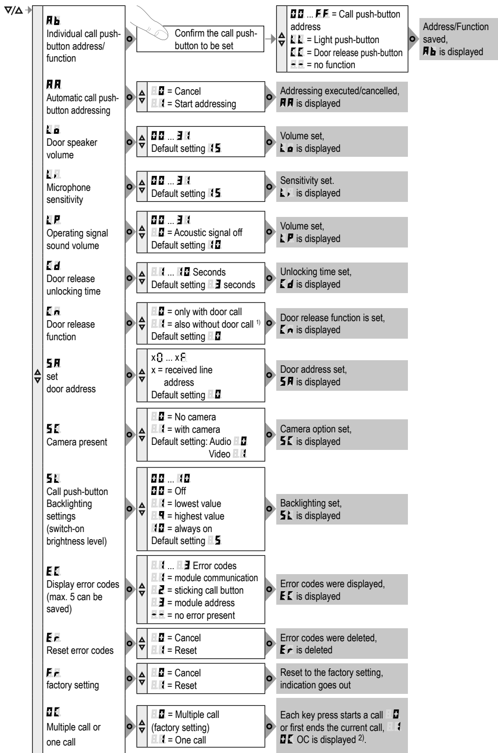
Figure 10: Overview of system settings
