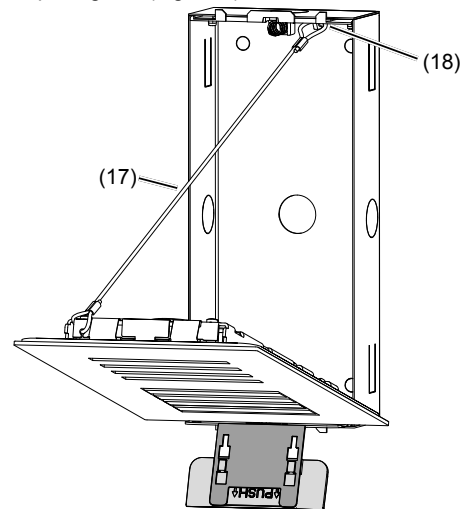
Figure 6: Installation position of door station
