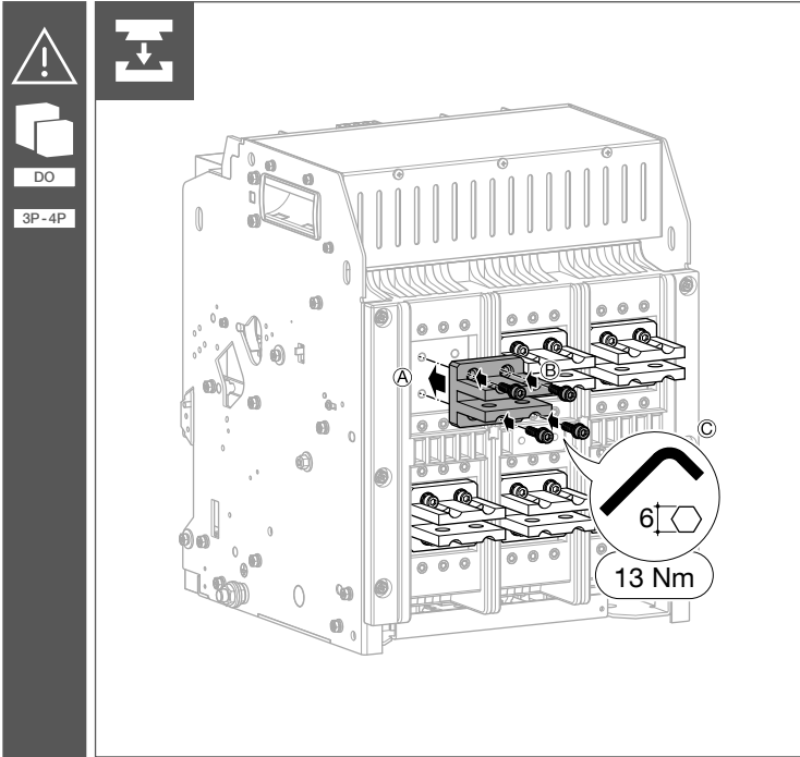
HW2 HWY162HSA (630 - 2500 A 3P) HWY163HSA (630 - 2500 A 4P)
